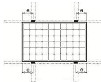
Figure2. Clamping on longer Frame
