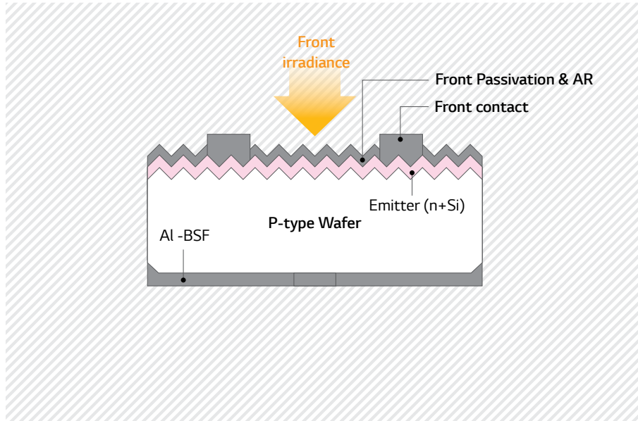
Monofacial (Conventional)
