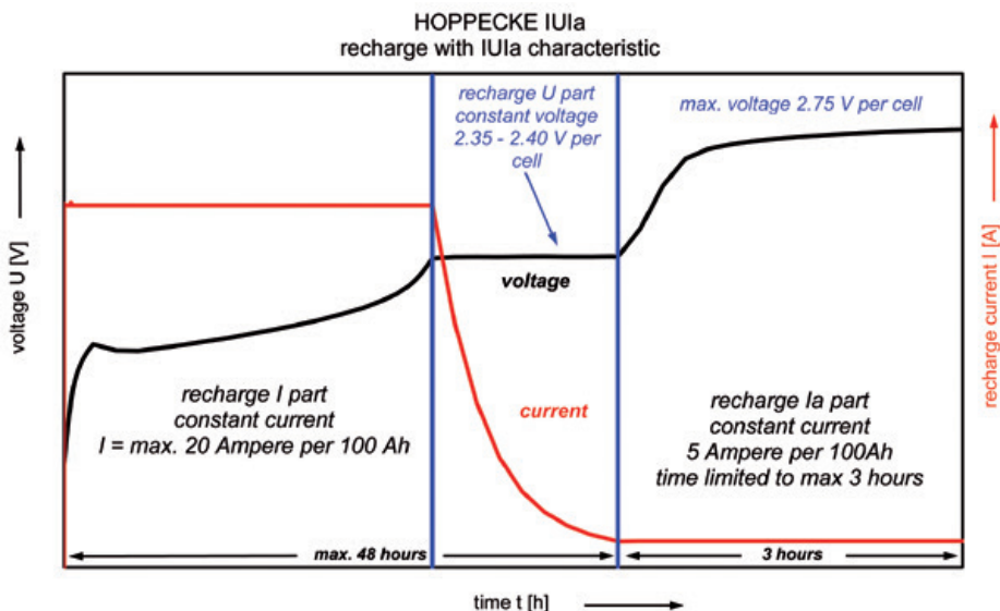
Fig. 9-2: IUla characteristic
