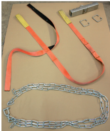
Fig. 5-4: Components of HOPPECKE hoisting belt
