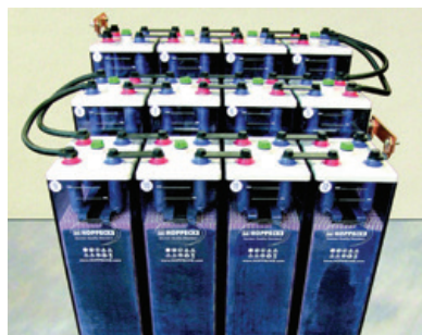
Fig. 5-16: Using row connectors and step connectors
