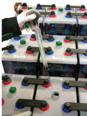
Fig. 6-2: Hydrometer
